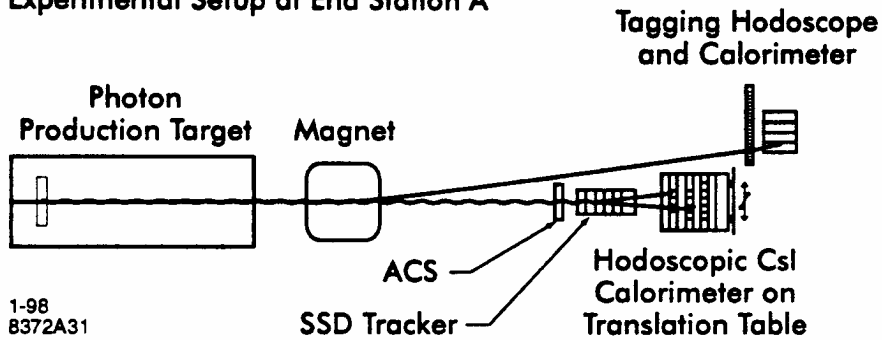
Experimental Setup at End Station A
