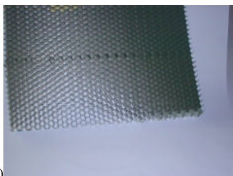
a) b) fig.1) MID012 honeycomb defect, entire view (a), close view (b). An extra wall all along a cell row is observed. Possible cause: bad cell gluing.
